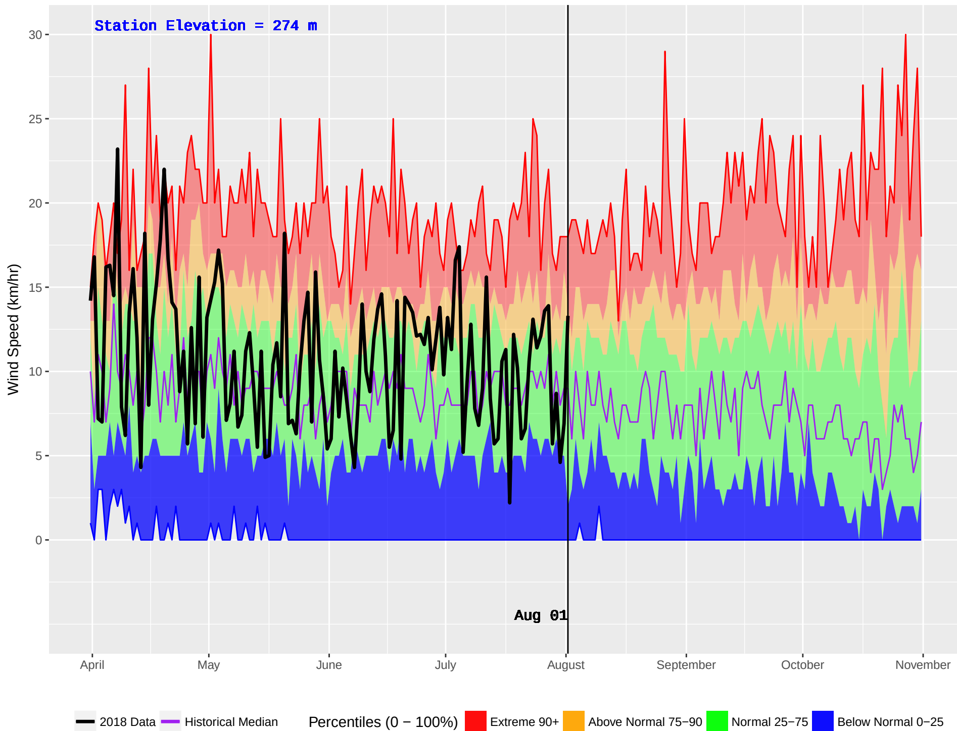
CEDARVALE (429) : Historical (1982–2016) and Current (2018) Daily Wind Speed
