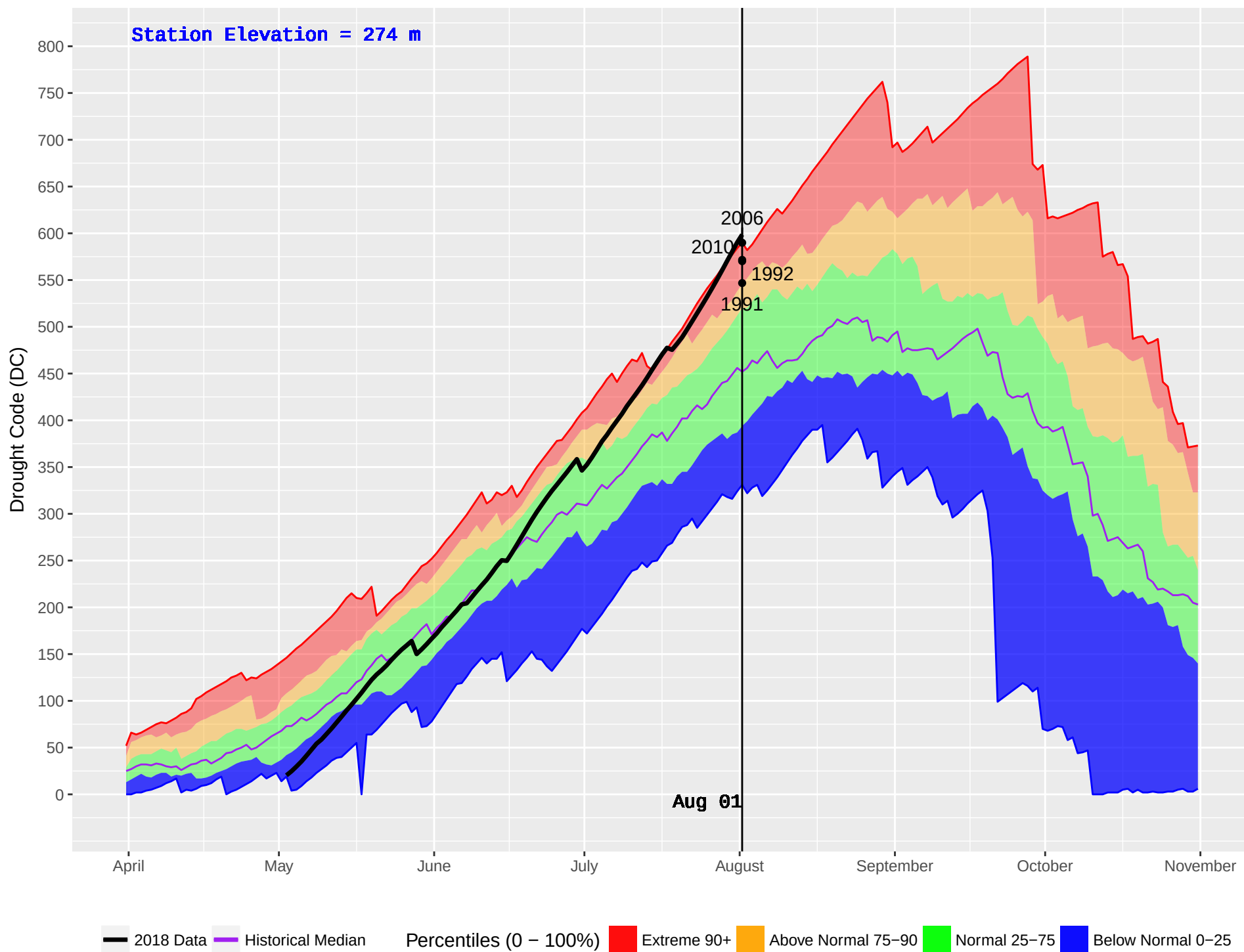
CEDARVALE (429) : Historical (1982–2016) and Current (2018) Daily Drought Code (DC)
