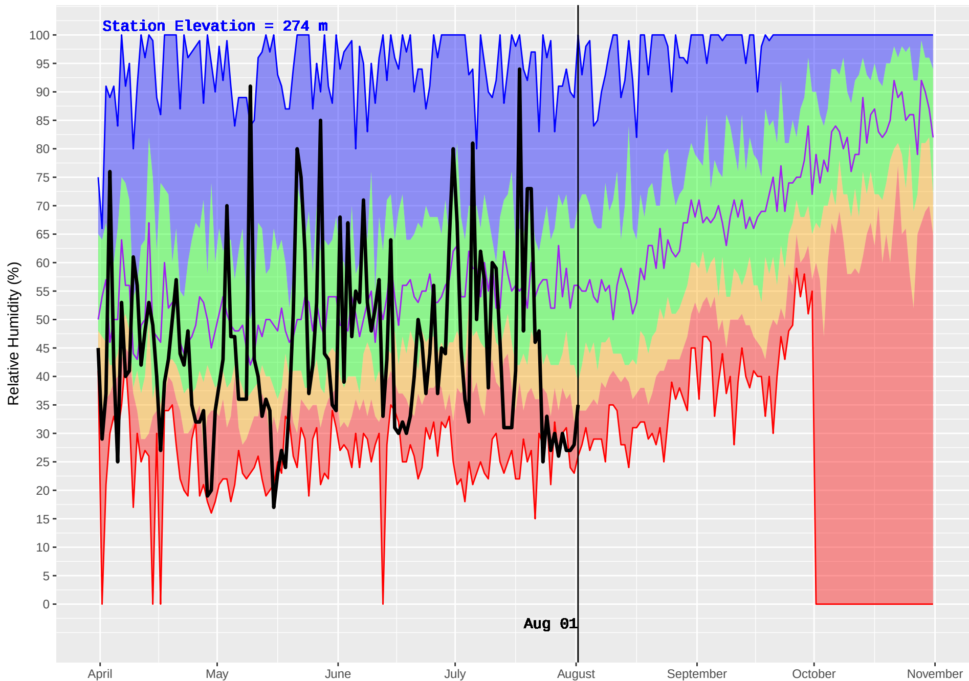
CEDARVALE (429) : Historical (1982–2016) and Current (2018) Daily Relative Humidity
